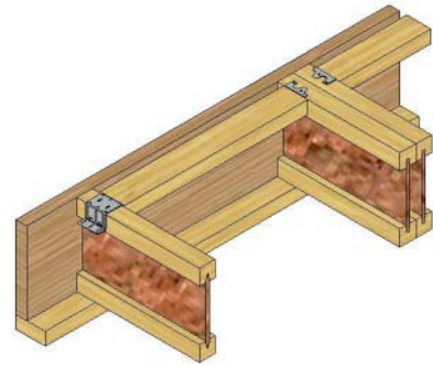
Minimum edge distance = 1¼" from centre of 1st nail to end of joist
