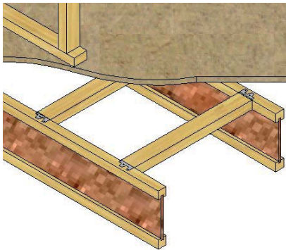
UZ clips supporting non-load bearing partition blocking
